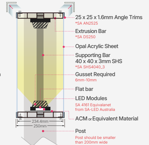
Side View : Fixed in between two posts
